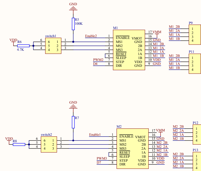
DRIVER_PART
